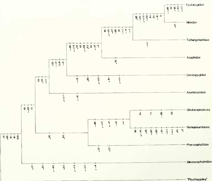
TEXT-FIG. 3. Another cladogram produced from the PAUP computer analysis of the characters given in Table 2, equally parsimonious with that shown in text-fig. 2. *, characters which are developed in parallel in more than one place on the cladogram; R, character reversals (i.e. advanced to primitive on Table 2); +, character transformations which we consider unlikely on other evidence (see text).
